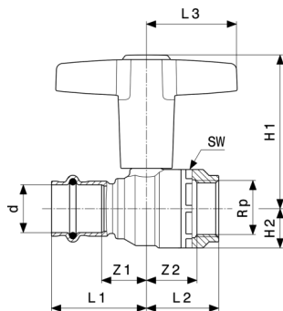
Easytop-Kugelhahn Modell 2275.4
