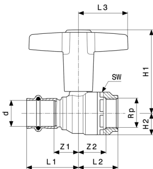
Easytop-Kugelhahn Modell 2275.4
