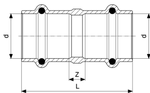
Sanpress-Muffe - Rotguss Modell 9777.9
