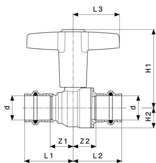
Easytop-Kugelhahn Modell 2275
