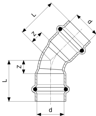
Sanpress Inox Elbow 45° - non-corroding steel Model 2326
