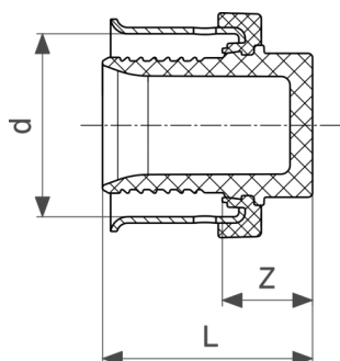
Viega Smartpress kap - PPSU model 4756
