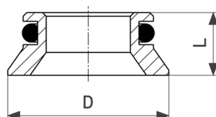
Adapterset model 1096.9
