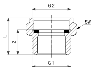
Adapterset - messing model 1022.7
