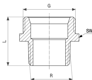
Overgangsstuknippel - brons of silicium brons model 3246
