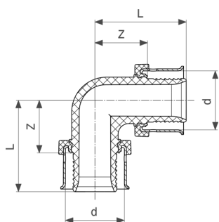
Viega Smartpress bocht 90° - PPSU model 4716
