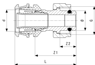
Raxofix-Adaptor - bronz siliconic model 5311.8
