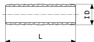
Hadicová spojka - mosadz model 1852
